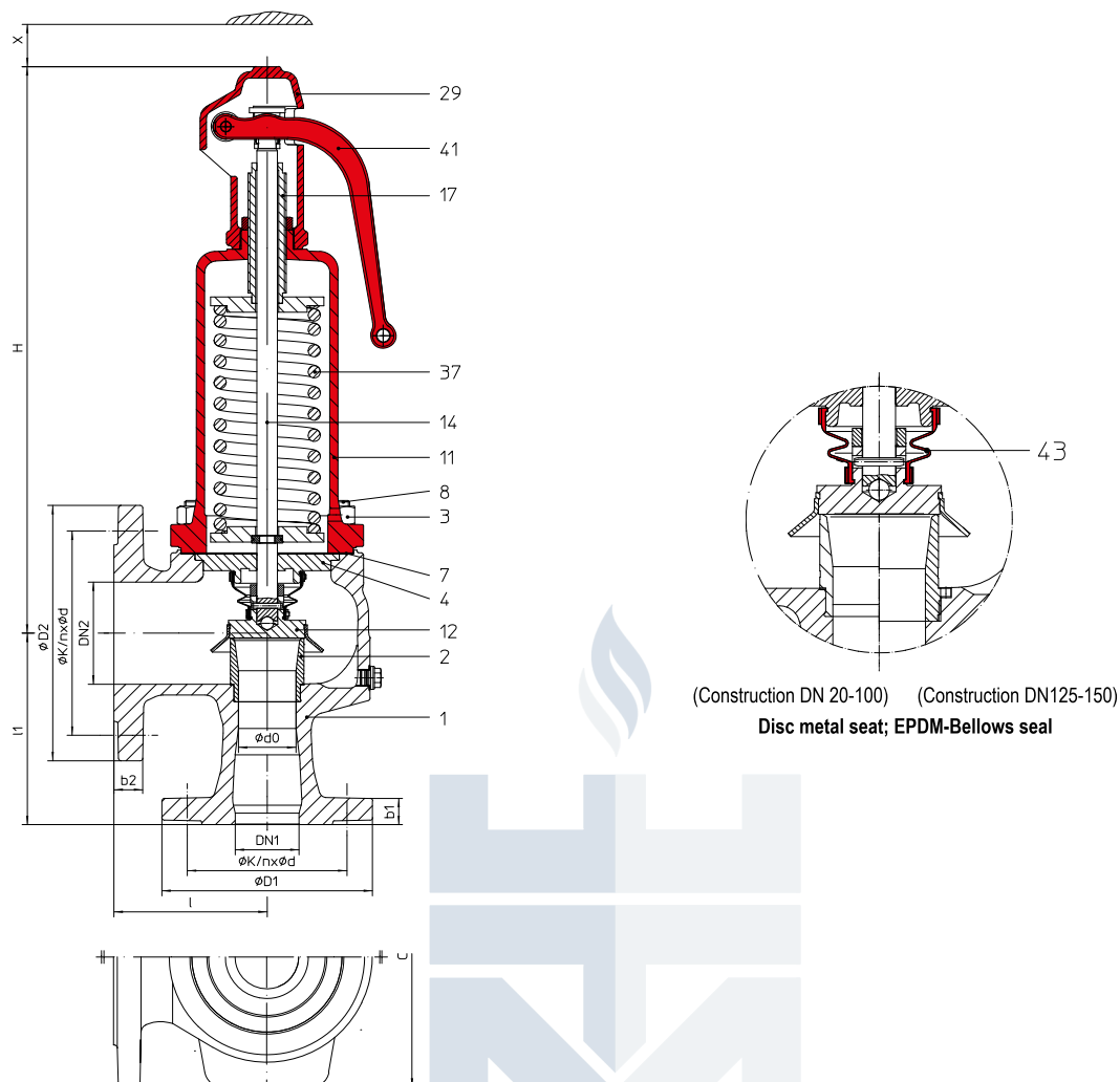
Fig. ... 904 open lifting device, closed bonnet
