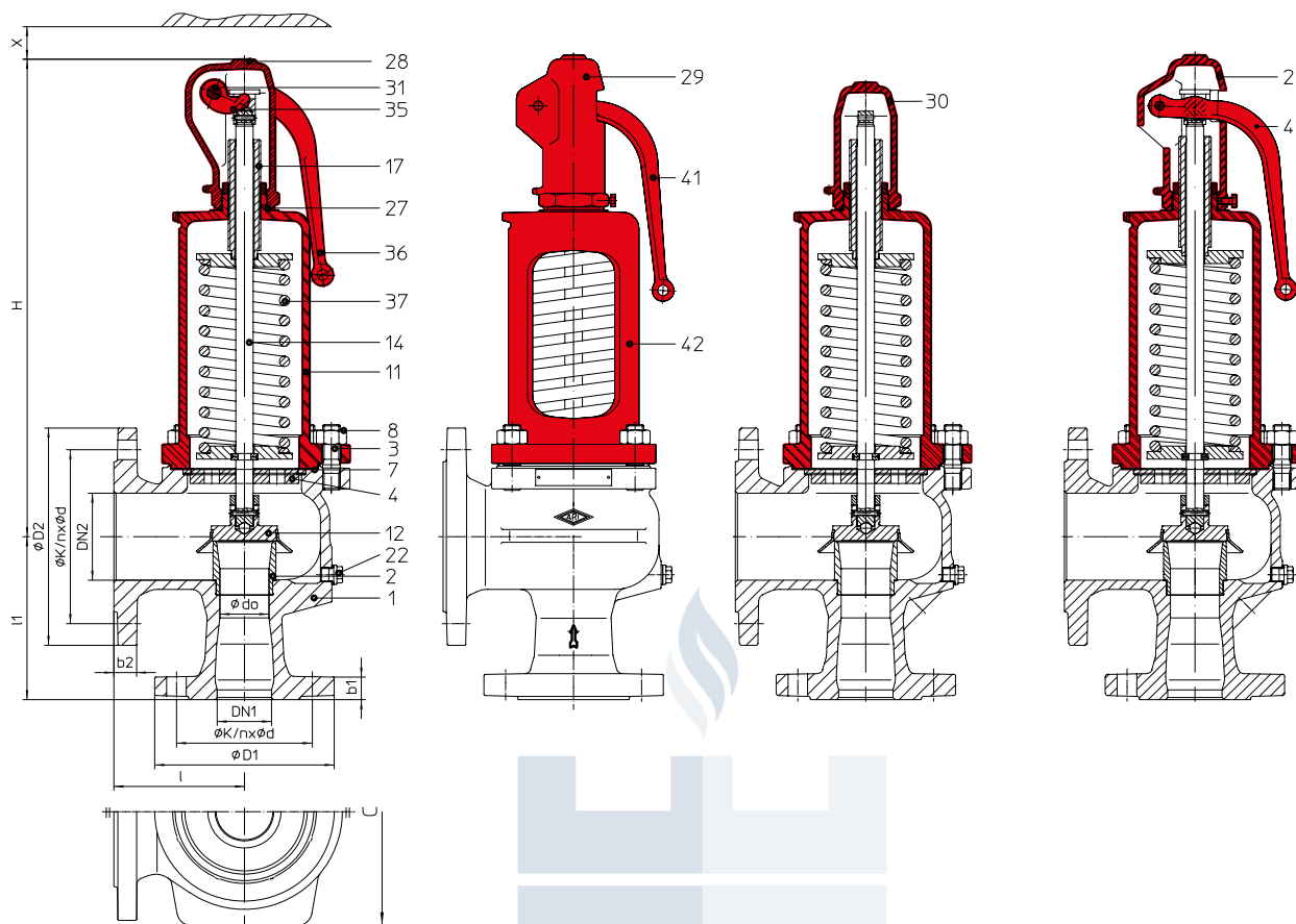
Fig. ... 901 closed lifting device, closed bonnet
