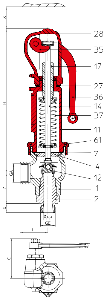
Fig. ... 941 closed lifting device, closed bonnet
