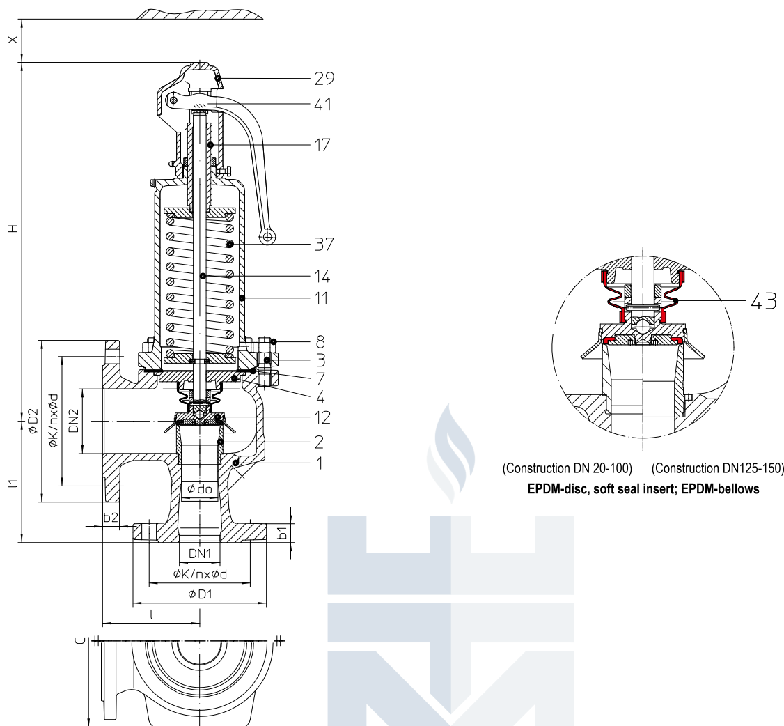
Fig. ... 903 open lifting device, closed bonnet
