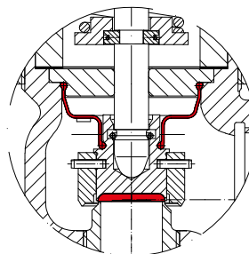
Fig. ... 945 EPDM-disc, soft seal insert; EPDM-bellows
