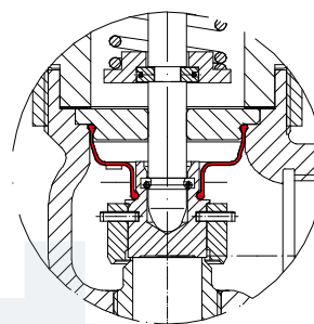
Fig. ... 946 Disc metal seat, EPDM-Bellows seal
