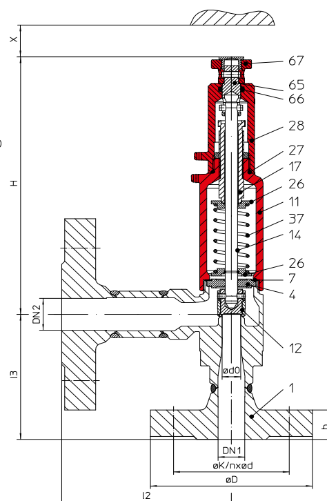
Fig. ... 961 / 962 / 963 optional with flange
