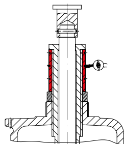
Lock bushing
