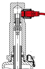
Proximity switch
