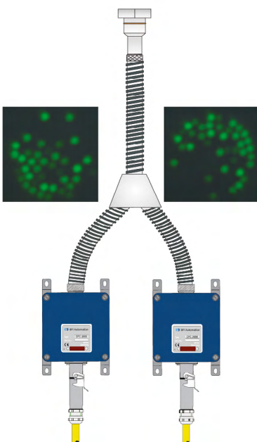
Splitting of one flame signal to two Flame Scanners / CFC.
