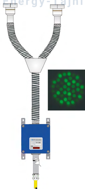
Merging of two flame signals to one Flame Scanner / CFC.
